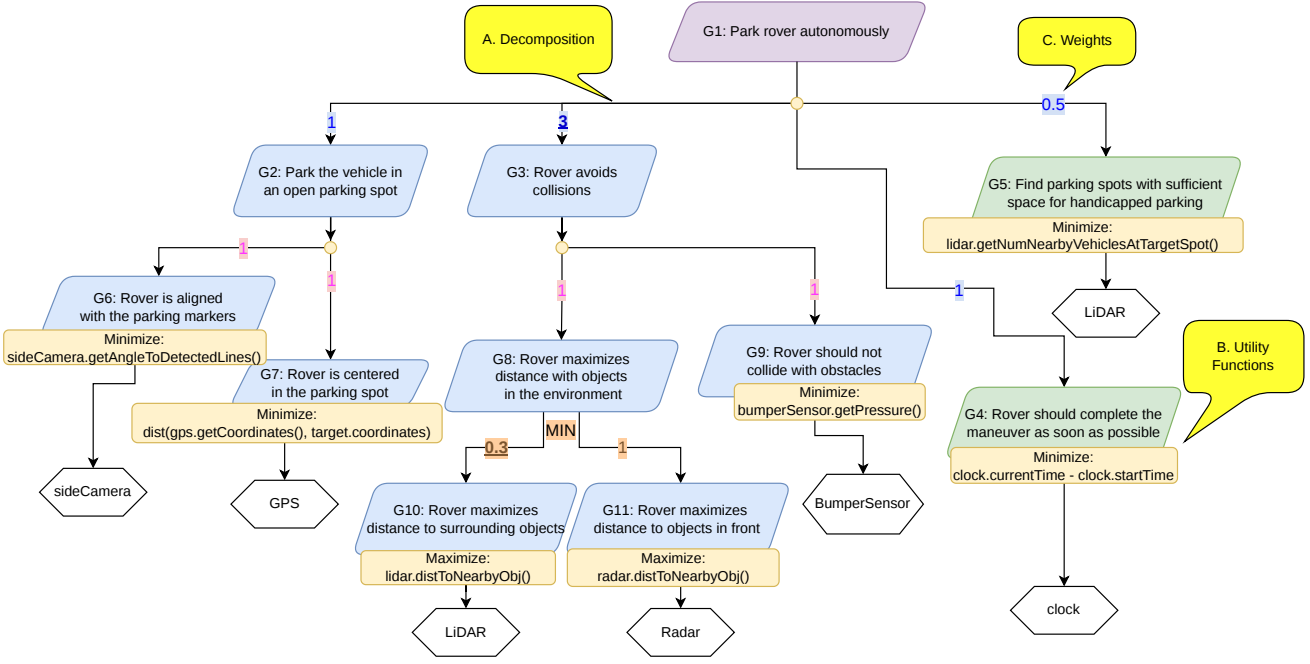
(a) The goal model used to decompose the abstract root objective of the rover into single requirements.
